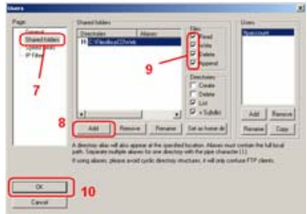
Figure E.c - FileZilla Server Interface: choosing the shared directory for "ftppaccount"
