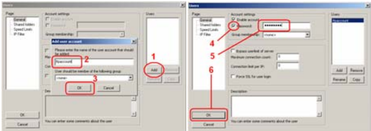
Figure E.b - FileZilla Server Interface: creating the "ftppaccount" user
